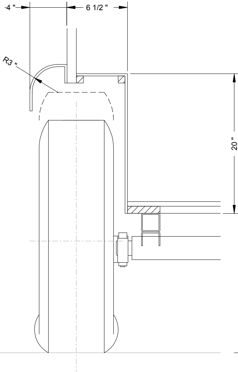
FIBERGLASS FENDER
